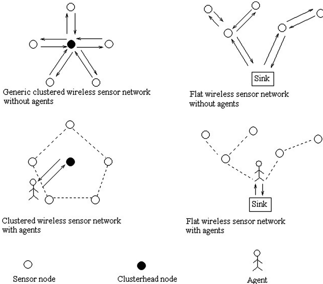
Figure 2: Mobile software agents.
